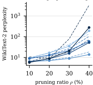
(a) language modelling
